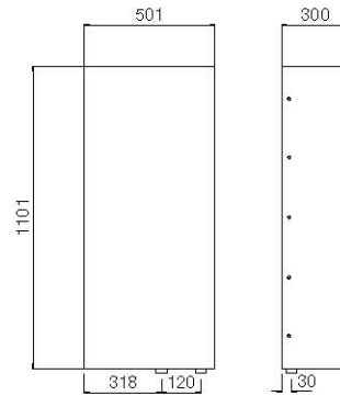
CONNECTIONS SIDE
